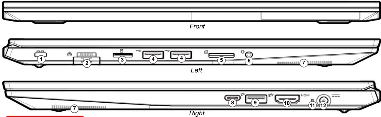
Figure 10 - Front, Left & Right Views (Model B)
